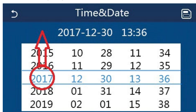
Time&Data Page
