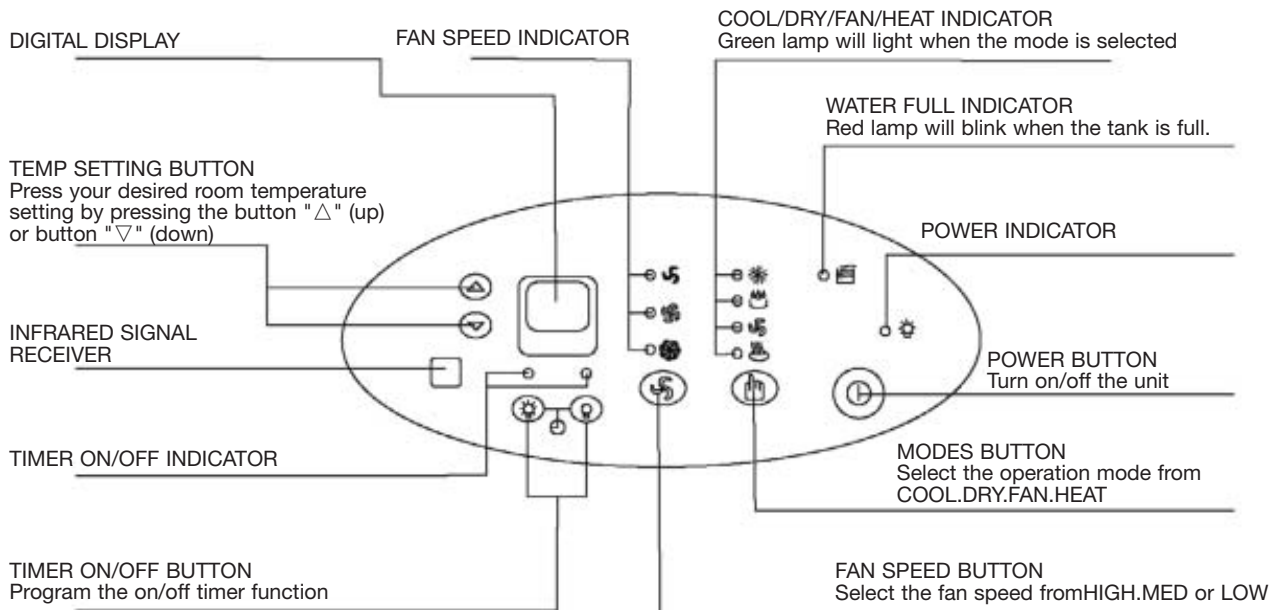
Operating panel
