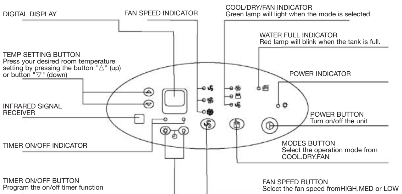
Operating panel
